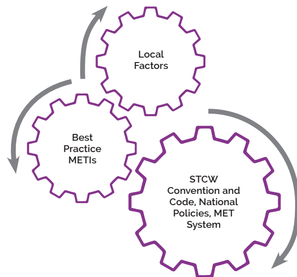
Figure 3: Compliance Framework
